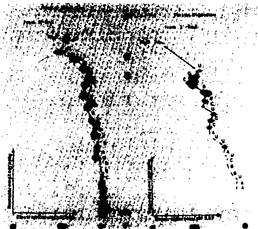
Fig. 9. Mobility shift analysis of the 20 mer (A) and 33 mer (B) using Homo-mix I. 31b
