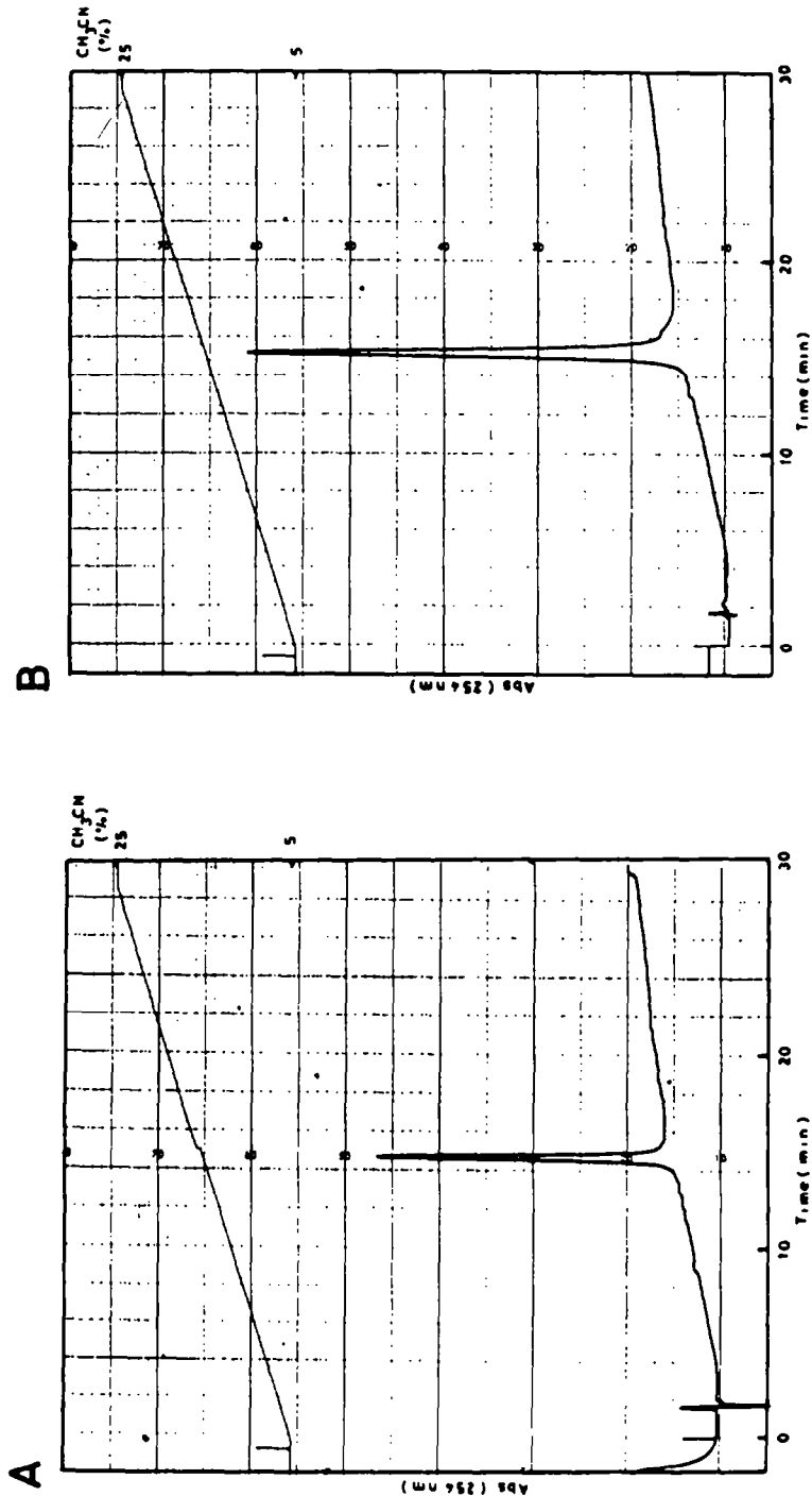
Fig. 7. Analysis of the purified 20 and 33 mer by HPLC on C-18 silica gel (TSK-LS410) in 0.1 M triethylammonium acetate.
